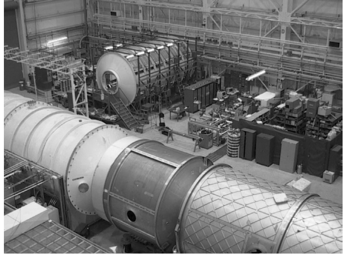
MSFC ECLSS Test Facility
